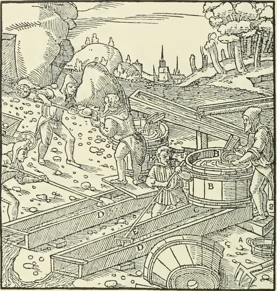
A—SIEVE. B—TUB. C—WATER FLOWING OUT OF THE BOTTOM OF IT. D—STRAKE. E—THREE-TOOTHED RAKE. F—WOODEN SCRUBBER.
